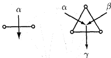
Fig. 2. Homomorphisms.
