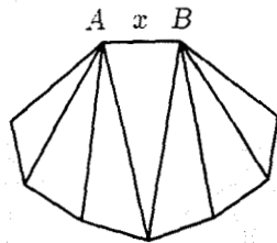
Fig. 5. A surface bimodule.
