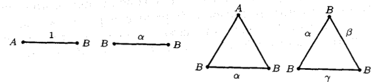
Fig. 14. Labels by \text{Rep}(G) .
