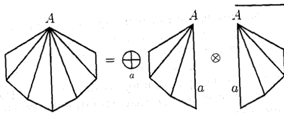
Fig. 4. A C^* -algebra \text{Alg}_n(A) .
