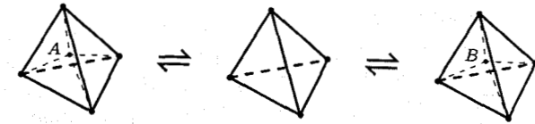
Fig. 12. Change of labels.
