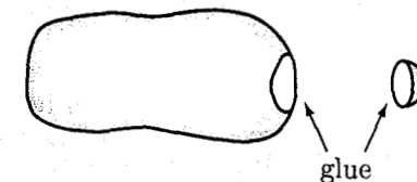
Fig. 15. 3-manifold with rind.
