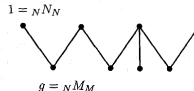
Fig. 1. An example of the principal graph.
