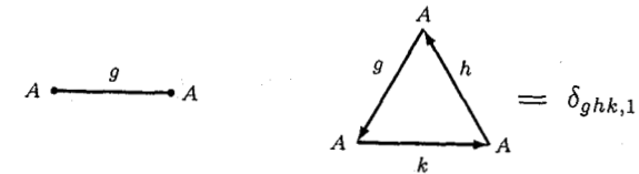
Fig. 13. Labels by G .
