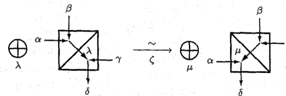
Fig. 3. Change of bases.
