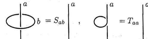
Fig. 34. S - and T -matrices.
