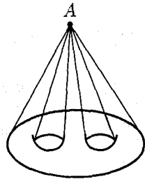
Fig. 16. A cone built over rind.
