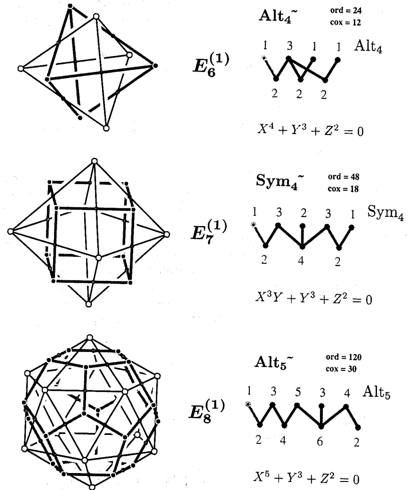
Fig. 29. Platonic solids and finite subgroups of SU(2) .
