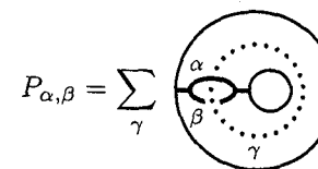
Fig. 11. An element in the center of Tube.
