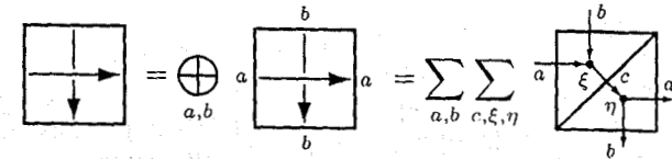
Fig. 6. A braiding.
