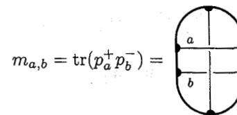
Fig. 40. A description of the modular invariant matrix.
