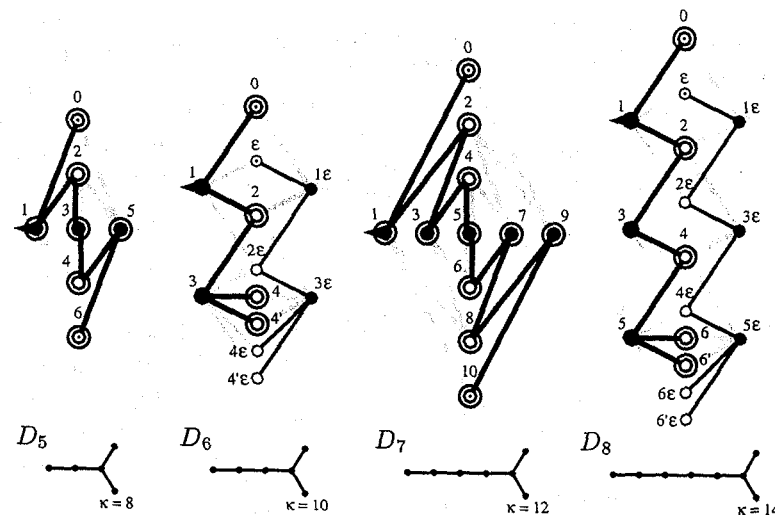
Fig. 21. Quantum symmetries for Coxeter graphs D_n .
