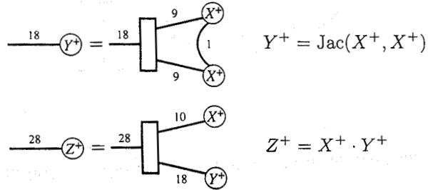
Fig. 31. The quantum Kleinian invariants of \text{QIcos}^+ .
