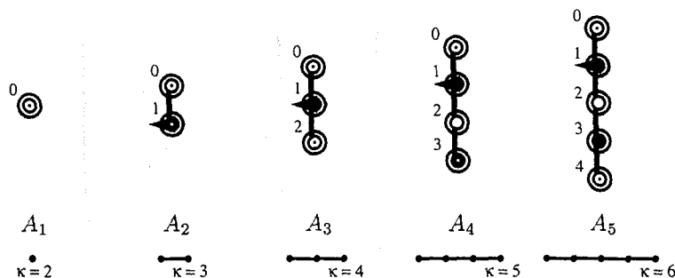
Fig. 20. Quantum symmetries for Coxeter graphs A_n .
