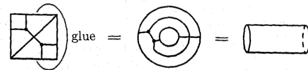
Fig. 7. Tube as a homomorphism.
