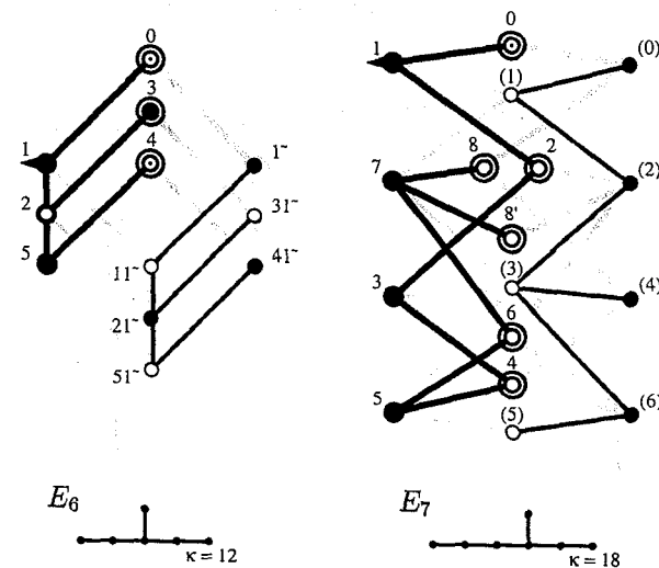
Fig. 22. Quantum symmetries for Coxeter graphs E_6 and E_7 .
