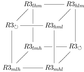
Figure 10: The cube of R3 moves.
