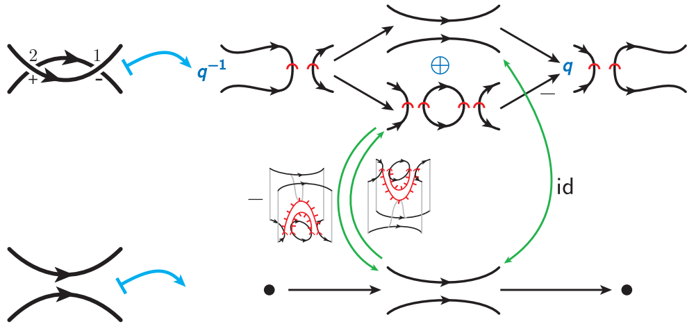
Figure 7: The R2a1 chain map. (The R2ar chain map is identical.)
