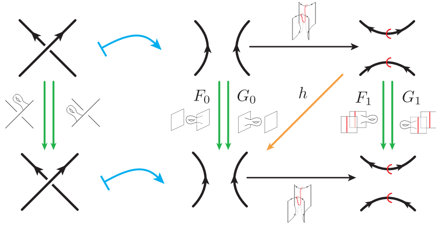
Figure 19: Chain maps and homotopy for the Proposition 4.6.
