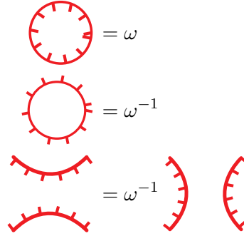
Figure 3: Disorientation relations.
