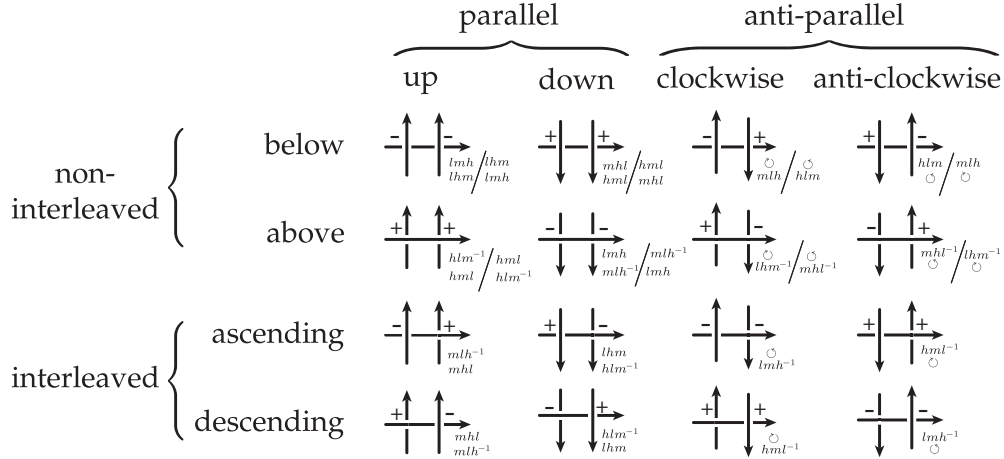
Figure 13: 16 variations for the initial frame of MM6.
