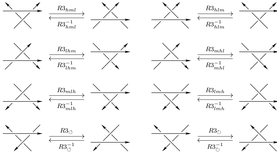
Figure 9: The eight variations of the R3 move. These diagrams are taken from [1]; they name the Reidemeister 3 moves differently, calling them III_a through III_h , reading across the rows.
