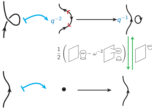
Figure 6: The R1b chain maps.
