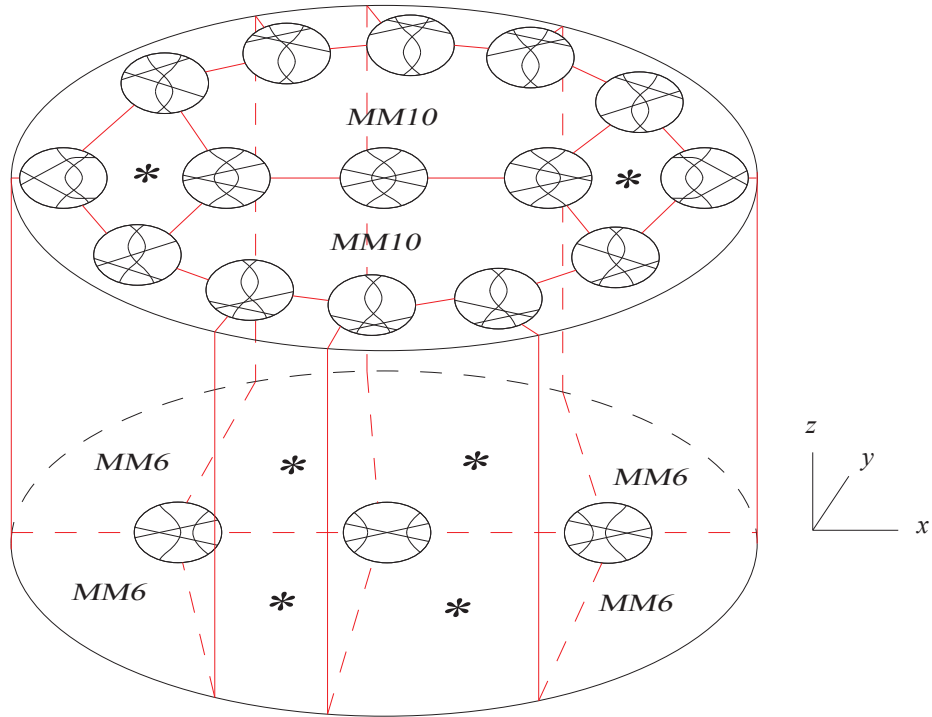
Figure 16: The 3-cell for the singularity in Figure 15, rotated 90 degrees. The 0-cells here are the generic tangle projections neighboring this singularity, achieved by untucking the curved strands ( z direction) and translating the crossing ( x and y directions). The 2-cells marked with an asterisk correspond to distant Reidemeister moves.
