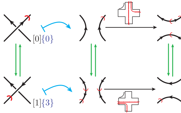
Figure 20: A hypothetical isomorphism of complexes implementing a particular case of the ‘vertigo’ move.
