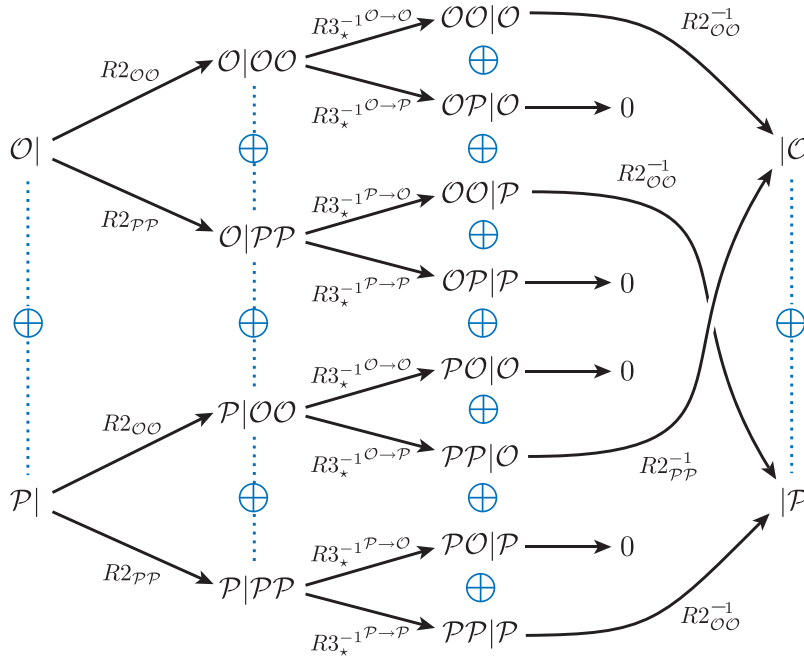
Figure 21: One R3 variation defined in terms of another via R2 moves.
