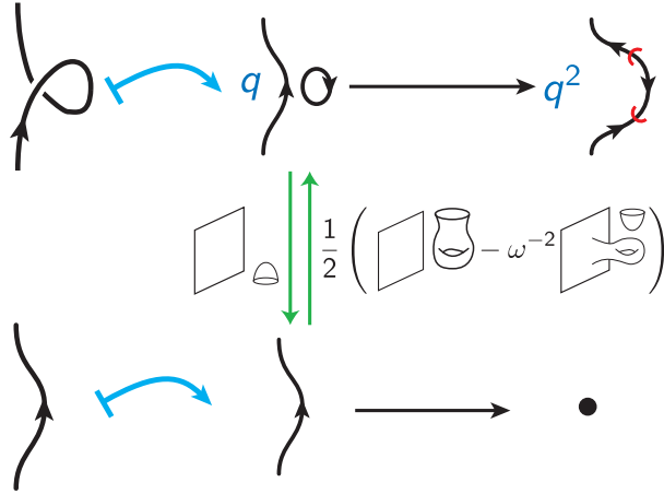
Figure 5: The R1a chain maps.
