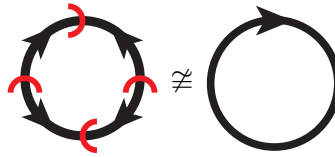
Figure 18: A disoriented circle with disorientation number +2 is not isomorphic in \mathbf{DisAb} to an oriented circle.
